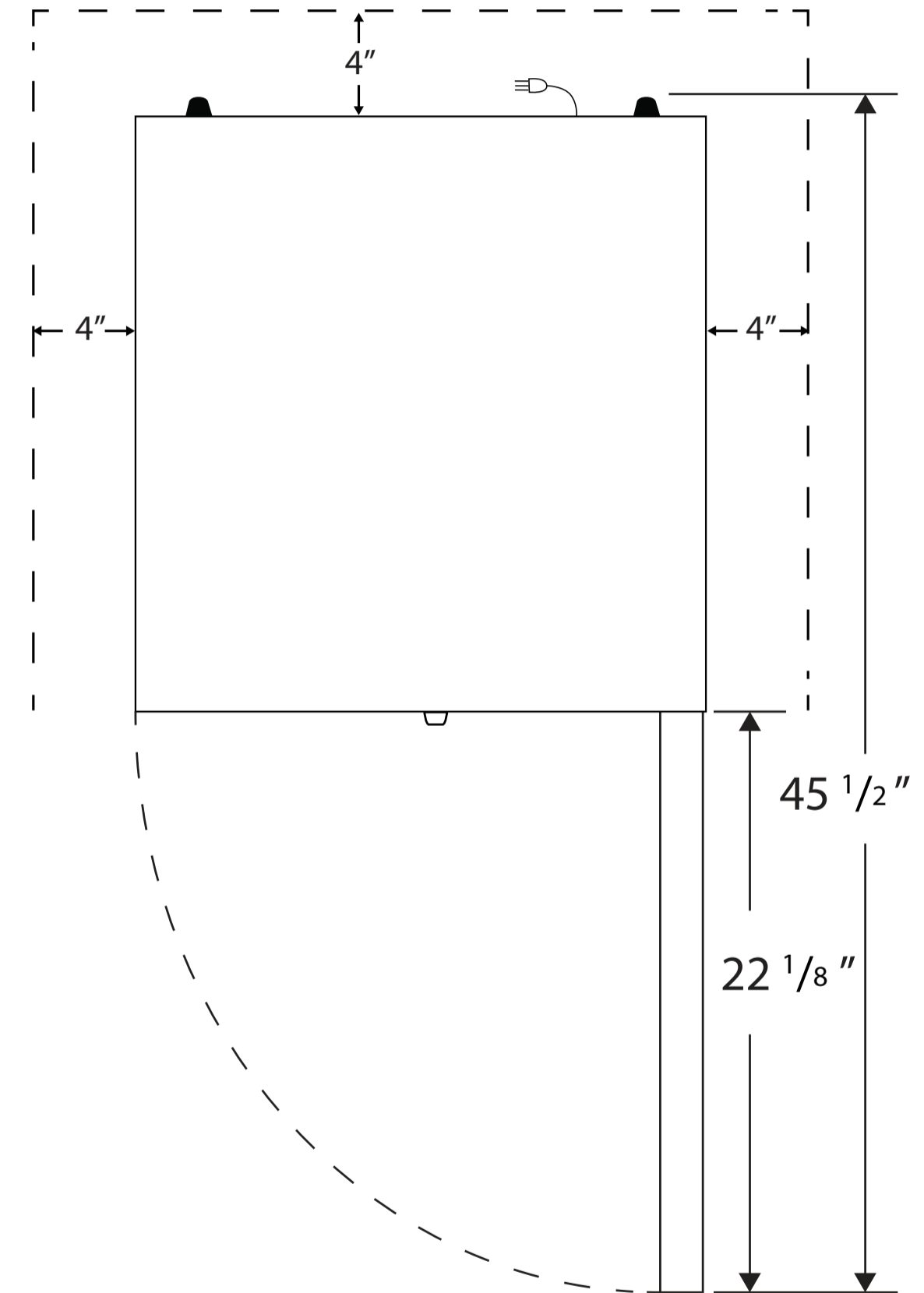
Top View
