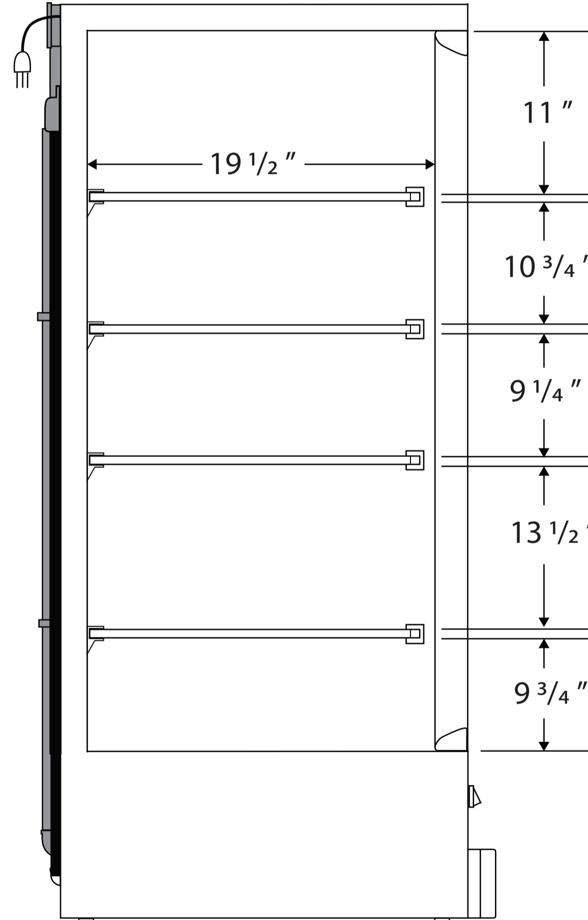
Side View
