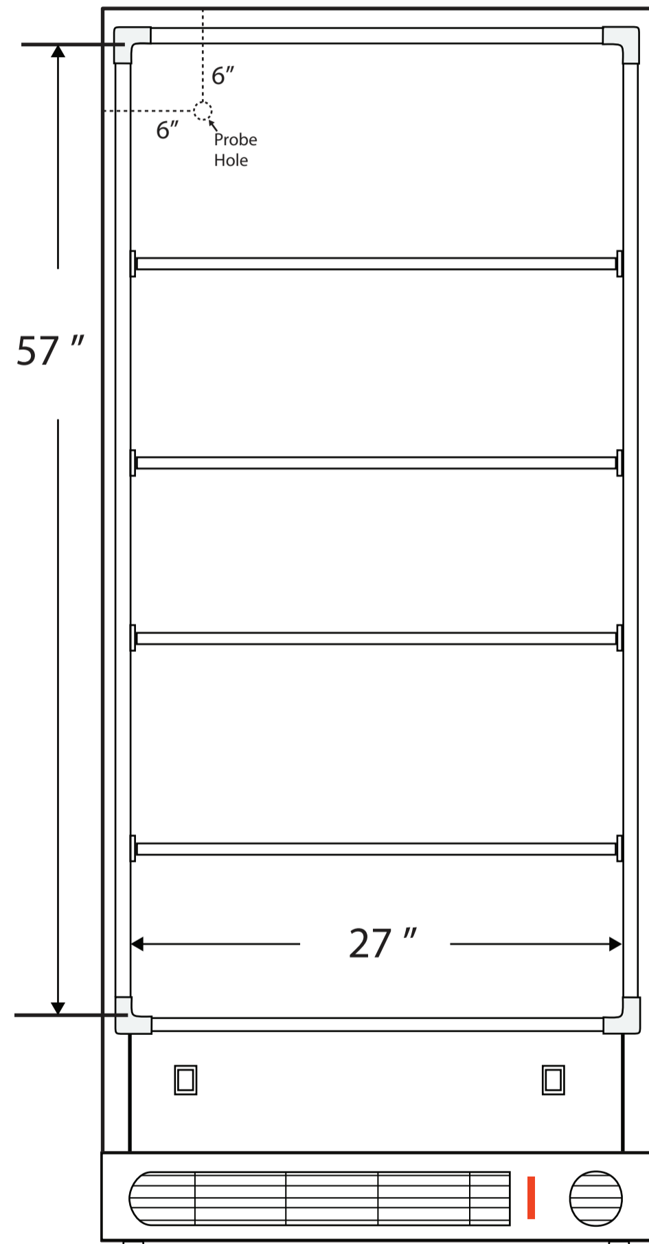
Front View
